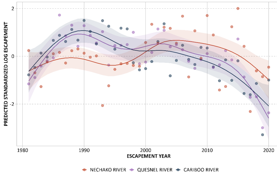
Figure 4. Observed (points) and predicted standardized log escapement (lines) for Nechako (red), Cariboo (black), and Quesnel (purple) rivers. Predicted values result from a GAM and shaded areas depict the 95% confidence intervals around predicted standardized log escapement.
